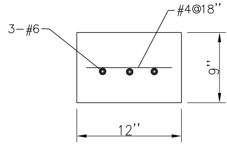
FOOTING DETAIL
